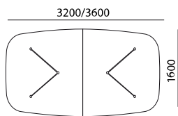
Tonel (sin/con top acces)
